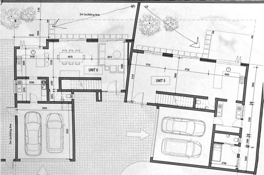
00 Ground Floor - Alternate Unit
