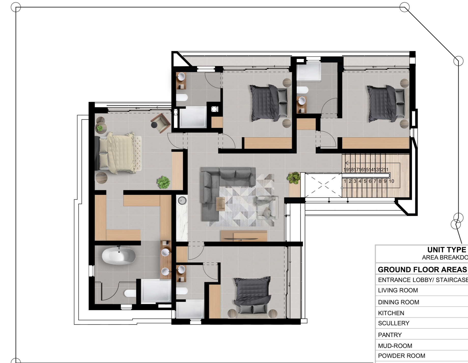
FIRST FLOOR Scale:1:100
